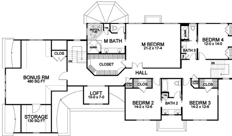
Second Floor
